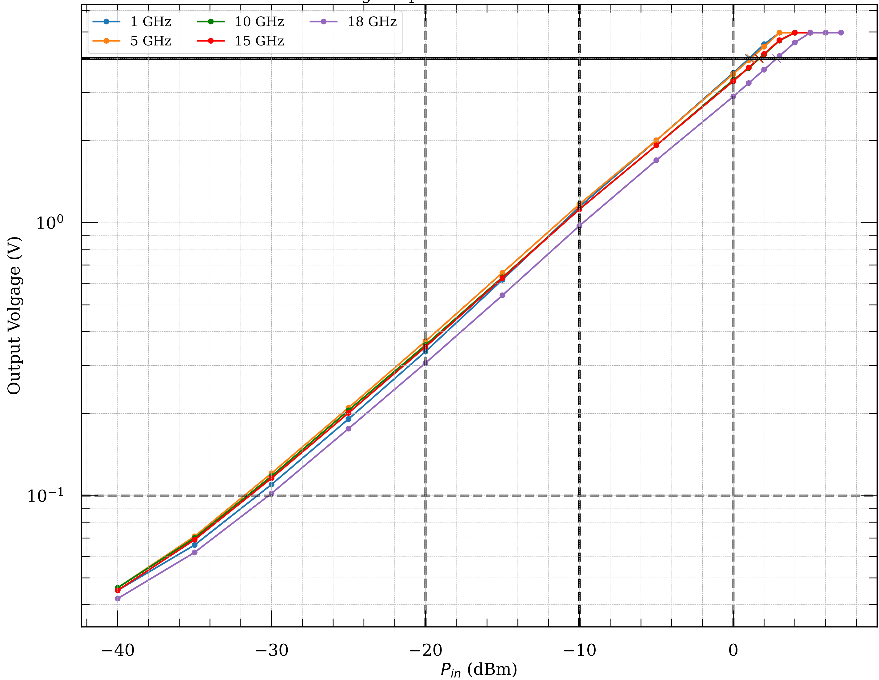
Measured voltage-to-power curve of detector module053v2
